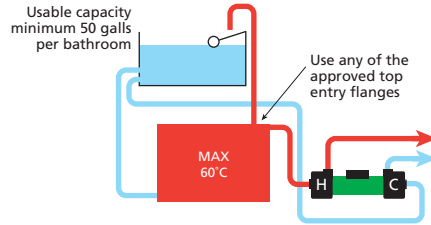
Figure 28: Horizontal cylinders
