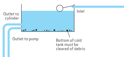
Figure 1: Tank inlet and outlet position
