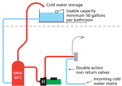
Figure 15: Tank fed (hot) with mains cold
