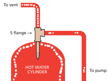
Figure 29: S flange
