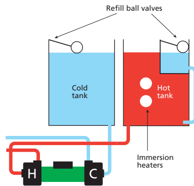
Figure 23: Elson (type) tanks
