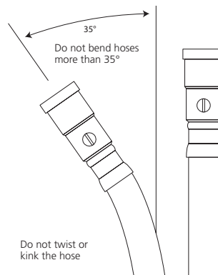
Figure 5: Couplers
